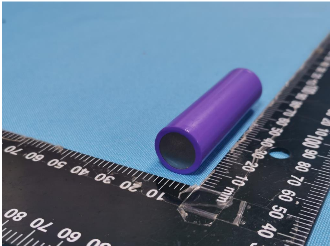
Picture 4. Bottom view of cell for model 18650 3.7V 2.0Ah 7.4Wh
