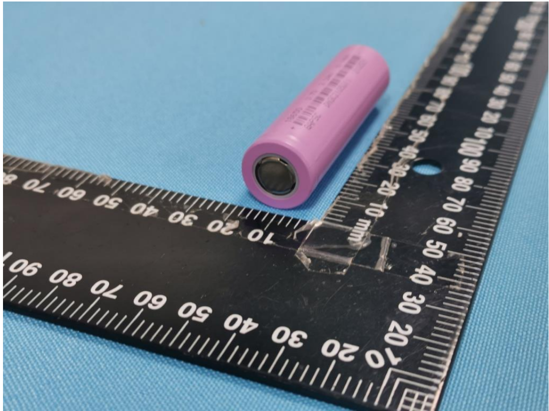
Picture 7. Top view of cell for model 18650 3.7V 2.2Ah 8.14Wh
