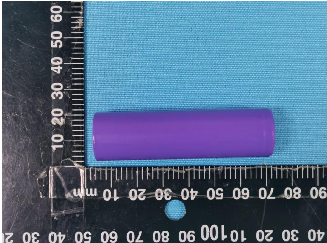
Picture 2. Back view of cell for model 18650 3.7V 2.0Ah 7.4Wh
